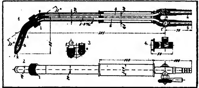
Fig. 1—Autogenous welding tool—dimensions in millimeters
